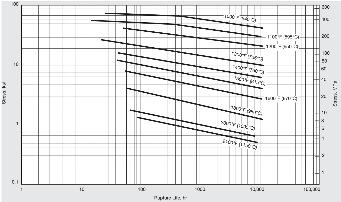
Figure 7. Typical rupture strength of solution-treated (2100°F) (1150°C) SOONV alloy 601.
