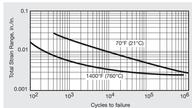
Figure 4. Low-cycle fatigue strength of SOONV alloy 601.
