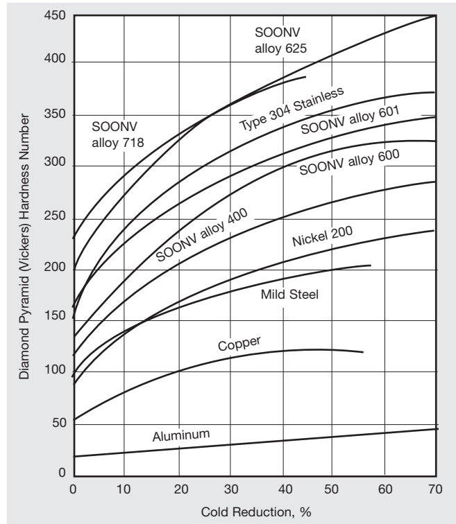
Figure 16. Work-hardening rates for SOONV alloy 601 and other materials.
