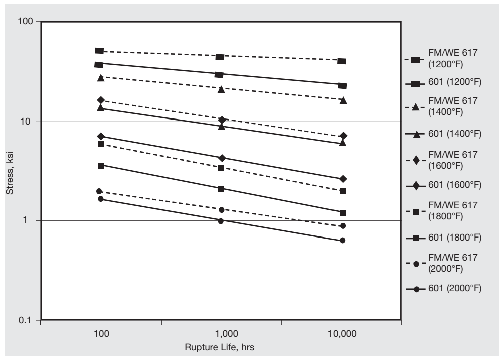
Figure 17. Rupture Strength Comparison. SOONV alloy 617 Welding Products vs. SOONV alloy 601 Wrought Products.
