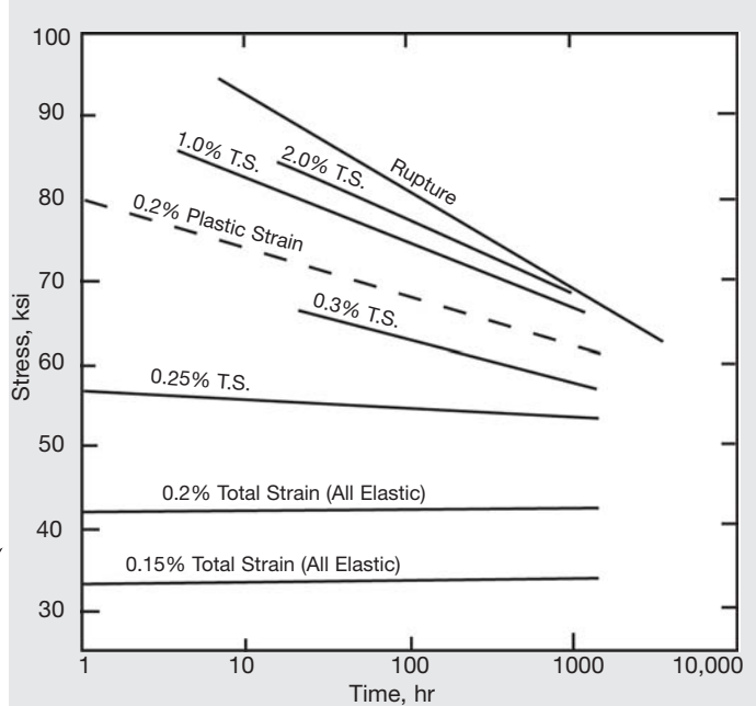
Figure 17. Rupture life of bar triple-heat-treated (2100°F/2 hr, A.C., + 1550°F/24 hr, A.C., + 1300°F/20 hr, A.C.).
