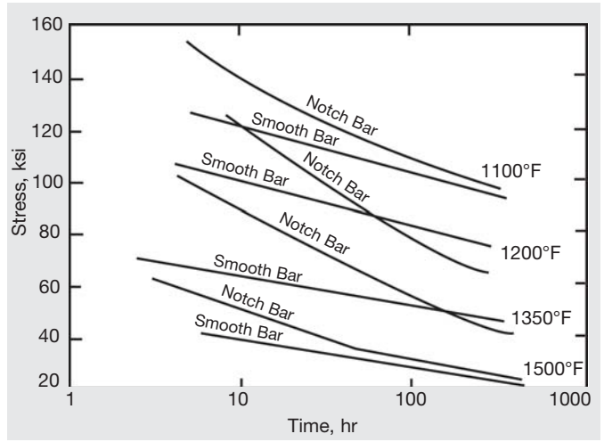
Figure 17. Rupture life of bar triple-heat-treated (2100°F/2 hr, A.C., + 1550°F/24 hr, A.C., + 1300°F/20 hr, A.C.).
