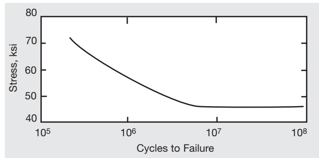
Figure 5. Fatigue strength of commercially produced SOONV alloy 400 wire (0.0375-in. diameter, cold-drawn 75% after final anneal). Tested in processed condition. Data determined with a rotating-wire (5000 rpm) arc-fatigue machine.
