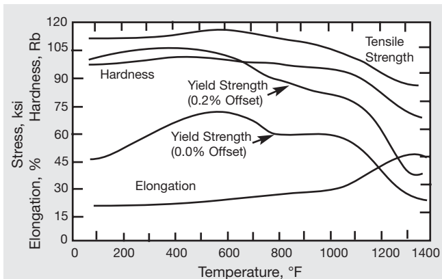
Figure 13. Effect of annealing (3 hr) on room-temperature properties of SOONV alloy 400 cold-drawn rod.
