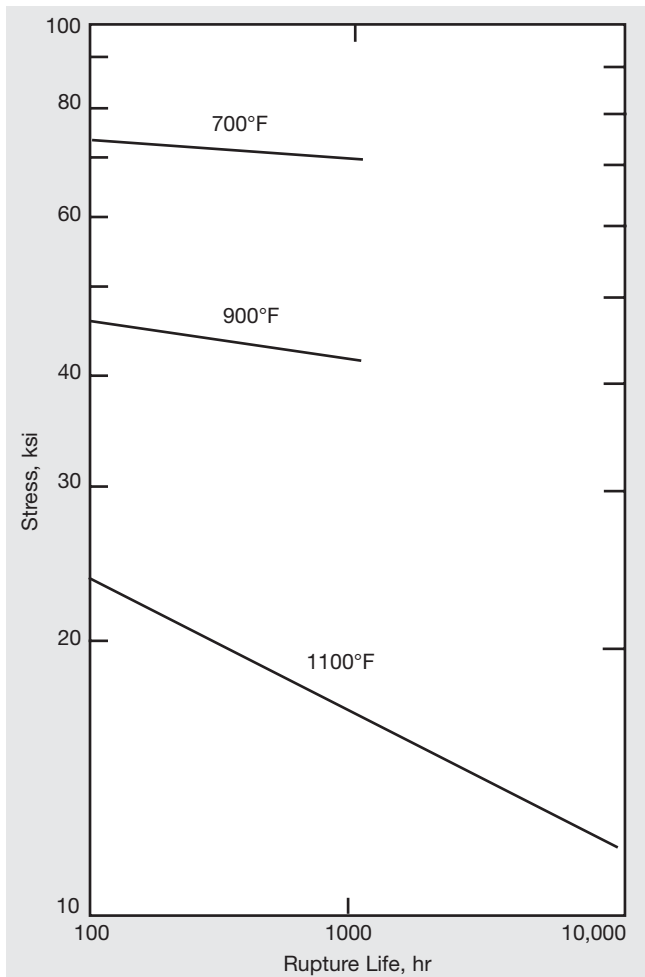
Figure 10. Rupture properties of cold-drawn annealed (1500°F/30 min) SOONV alloy 400.
