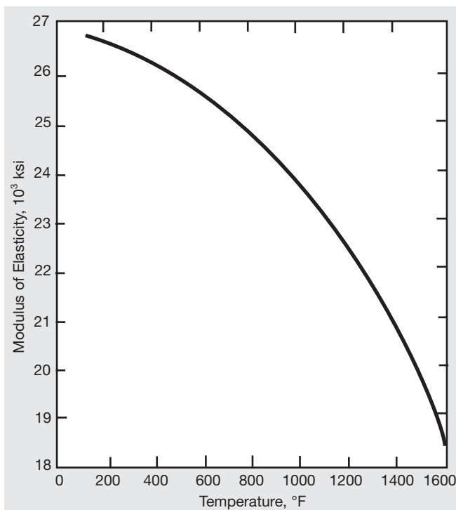
Figure 1. Effect of temperature on modulus of elasticity in tension of Soonv alloy 400 (determined by dynamic method).
