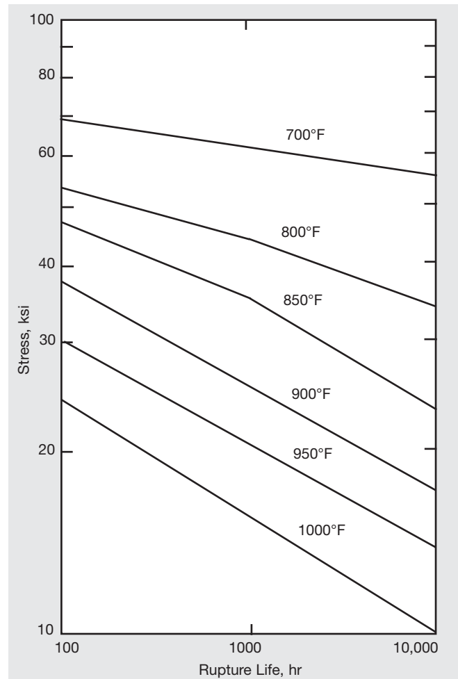
Figure 11. Rupture properties of cold-drawn, stress-relieved (1100°F/8 hr) SOONV alloy 400.
