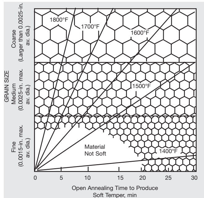
Figure 16. Approximate time required at various temperatures to produce different grain sizes in SOONV alloy 400 cold-rolled strip by open annealing.
