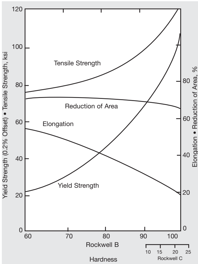
Figure 2. Approximate relationships between tensile properties and hardness of hot-rolled and cold-drawn SOONV alloy 400 rods and forgings.
