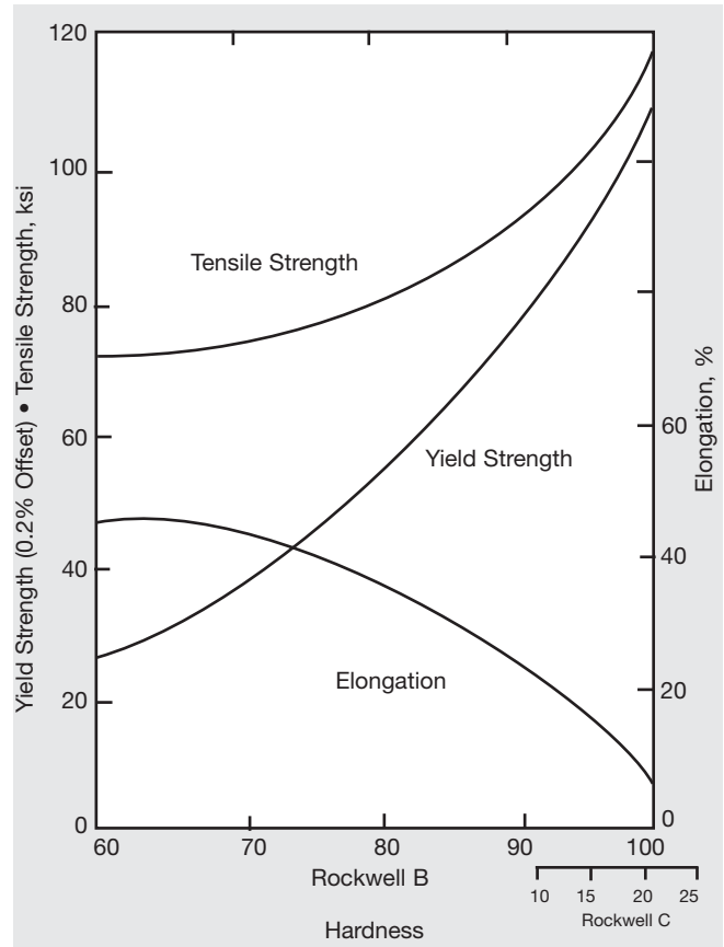
Figure 3. Approximate relationships between tensile properties and hardness of SOONV alloy 400 sheet and strip.
