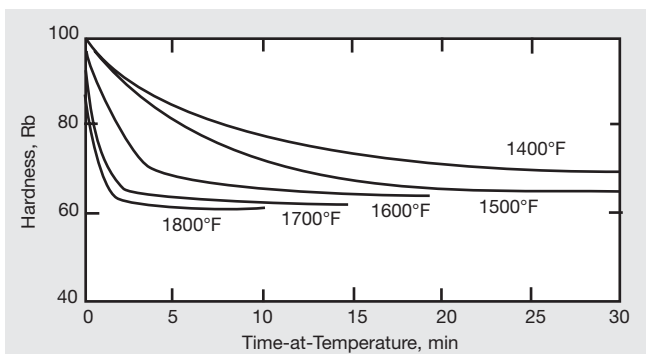
Figure 15. Approximate time required at various temperatures to produce different hardness levels in SOONV alloy 400 cold-rolled strip by open annealing.
