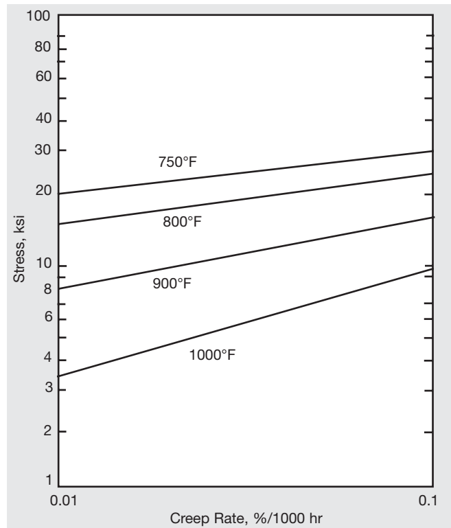
Figure 8. Creep properties of cold-drawn annealed (1500°F/3 hr) SOONV alloy 400.
