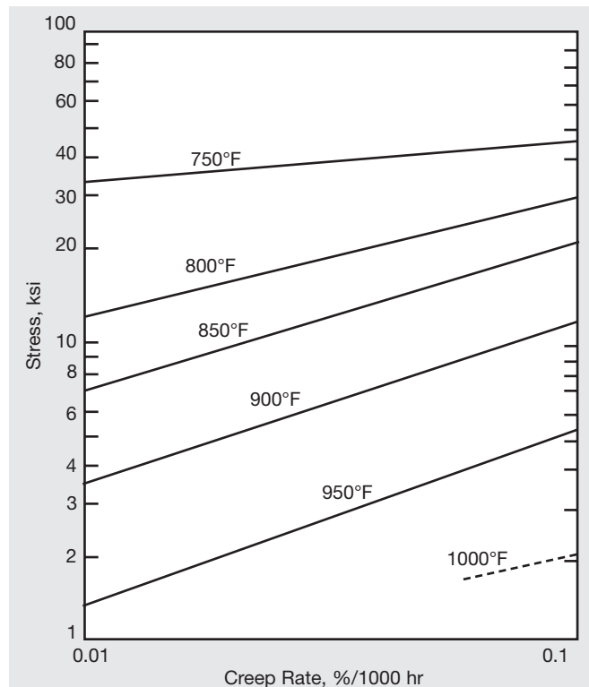
Figure 9. Creep properties of 20% cold-drawn stress-relieved (1000°F/8 hr) SOONV alloy 400.
