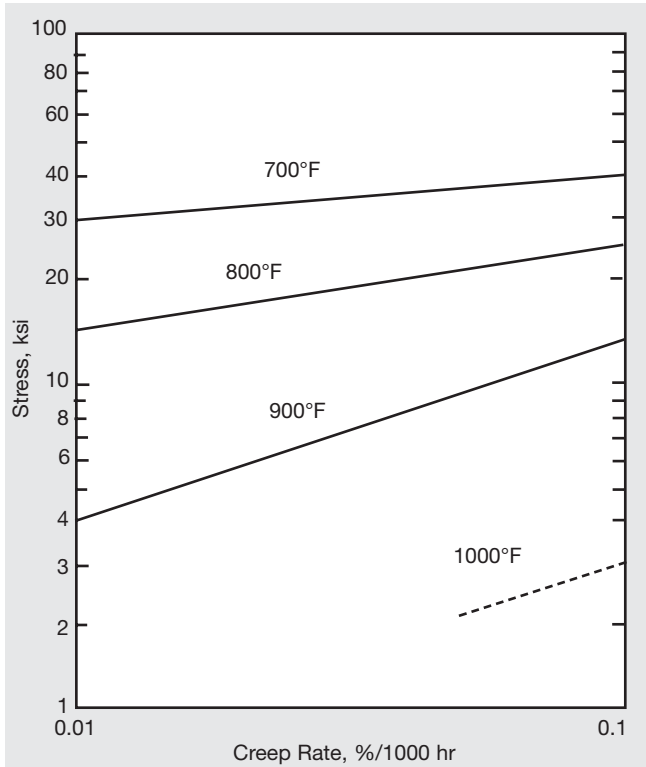
Figure 7. Creep properties of hot-rolled SOONV alloy 400.
