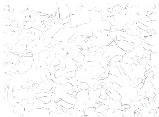
Figure 12. Longitudinal section of cold-drawn SOONV alloy 400 rod. Etchant: Sodium cyanide--ammonium persulfate. 100X.
