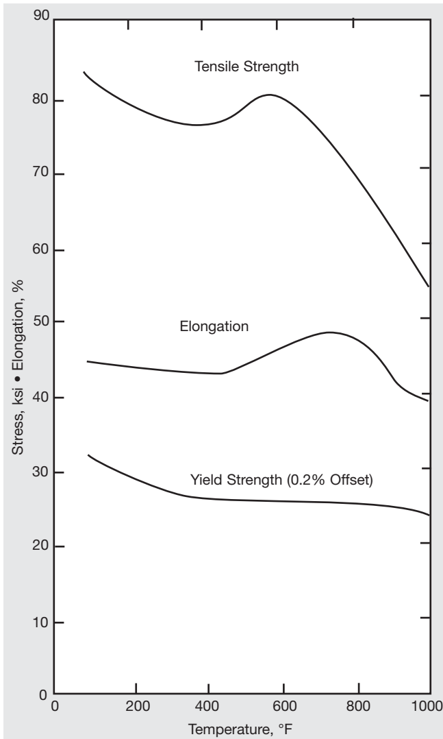
Figure 4. High-temperature properties of annealed SOONV alloy 400.
