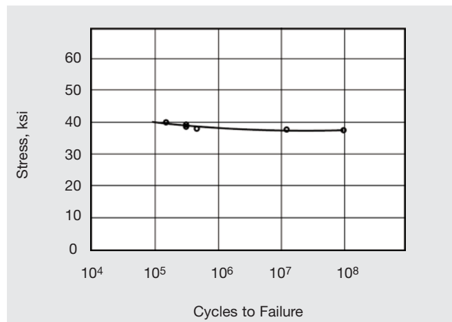
Figure 6. Fatigue strength of commercially produced SOONV alloy 400 rod (0.500-in. diameter, cold-drawn, annealed 1500°F/3 hrs). Tested in the processed condition. Data determined by the R.R. Moore rotating beam technique.
