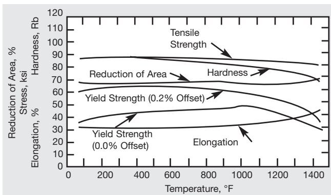
Figure 14. Effect of annealing (3 hr) on room-temperature properties of hot-rolled SOONV alloy 400 plate. At 1470°F, material is fully annealed. (Hardness converted from BHN.).
